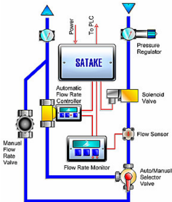
Diagram of SWEC Panel with Litres/Minute Controller
